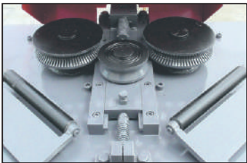
One step radius bending process
